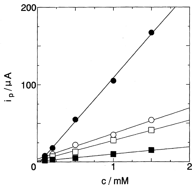
Fig. 3. Dependence of peak currents at poly-MPP-coated GC electrode (●, ■) and naked GC electrode (○, □) on the concentration of quinhydrone in a 0.2 M Na 2 SO 4 –0.01 M H 2 SO 4 solution. Circles, anodic peak; squares, cathodic peak. Scan rate = 100 mV s –1 .
