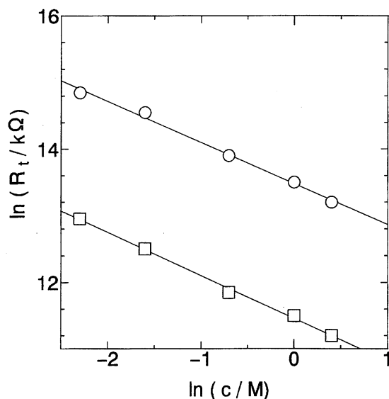
Fig. 6. Changes in charge-transfer resistances at naked GC electrode (○) and poly-MPP-coated GC electrode (□) with the quinhydrone concentration in a 0.2 M Na 2 SO 4 –0.01 M H 2 SO 4 solution. Applied potential: 0.36 V.
