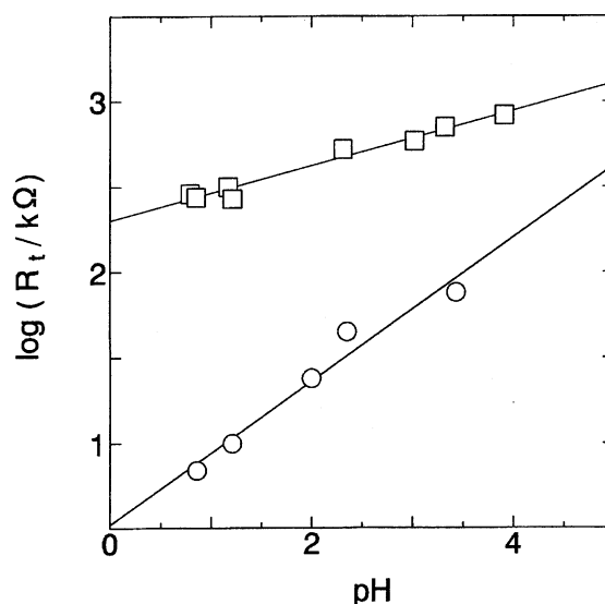
Fig. 8. Charge-transfer resistances at poly-MPP-coated GC electrode (○) and naked GC electrode (□) as a function of the pH of a Na 2 SO 4 solution containing 1 mM quinhydrone.
