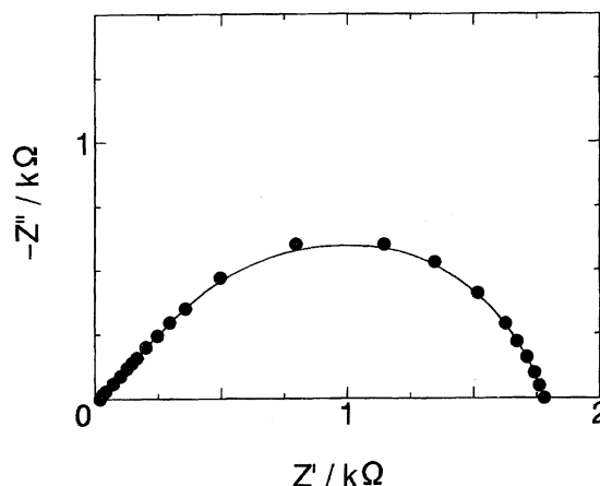
Fig. 10. Typical impedance plots for a metal/film/metal cell where the film is in contact with a 0.2 M \text{Na}_2\text{SO}_4 –0.01 M \text{H}_2\text{SO}_4 solution. After the polymer film had been equilibrated at 0.39 V, the impedances of the cell were measured.
