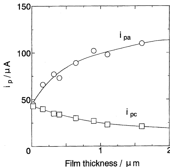
Fig. 9. Dependence of anodic peak current (○) and cathodic peak current (□) on film thickness. Cyclic voltammograms were measured at a scan rate of 200 \text{ mV s}^{-1} in a 0.2 M \text{Na}_2\text{SO}_4 –0.01 M \text{H}_2\text{SO}_4 solution containing 1 mM quinhydrone.
