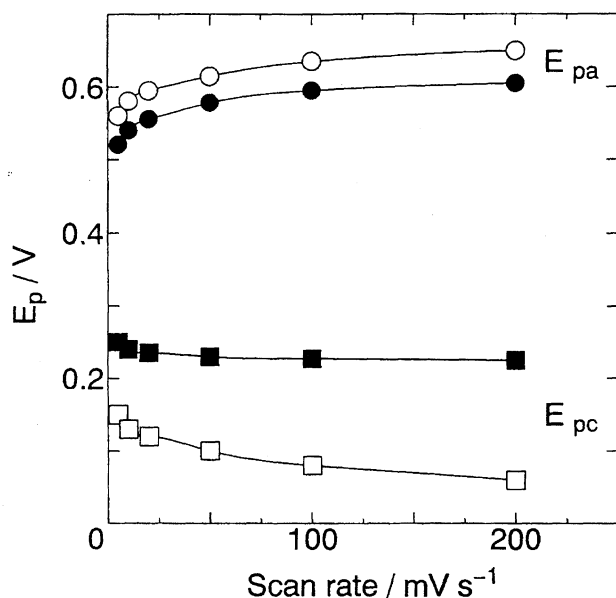
Fig. 2. Peak potentials of quinhydrone at poly-MPP-coated GC electrode (●, ■) and naked GC electrode (○, □). Circles, anodic peak; squares, cathodic peak.
