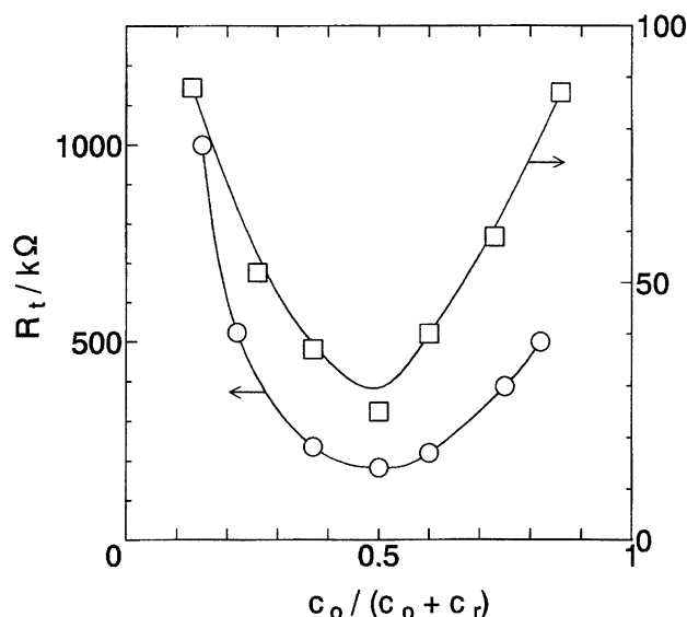
Fig. 7. Relationship between R_t and the composition of redox couple in a 0.2 M Na 2 SO 4 –0.01 M H 2 SO 4 solution. Circles, naked GC electrode; squares, poly-MPP-coated GC electrode. Impedances were measured at each equilibrium potential. The total concentration of redox couple is 1 mM.
