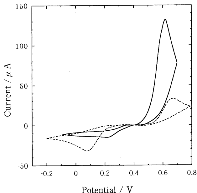
Fig. 1. Cyclic voltammograms of poly-MPP-coated GC electrode (—) and naked GC electrode (---) in a 0.2 M Na 2 SO 4 –0.01 M H 2 SO 4 solution containing 1 mM quinhydrone. Scan rate = 100 mV s -1 .
