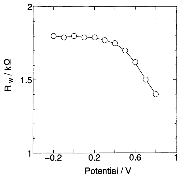
Fig. 11. Change in R_w with electrode potential.
