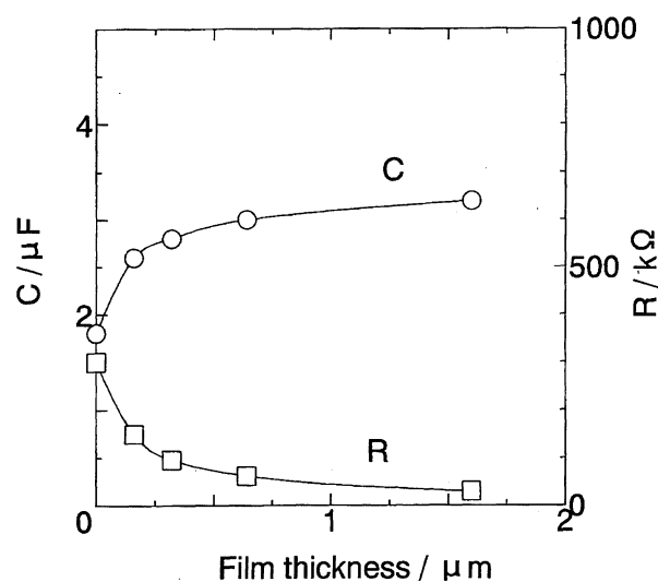
Fig. 5. Changes in the diameter of semicircle (□) and capacitance (○) with film thickness. Applied potential: 0.36 V.
