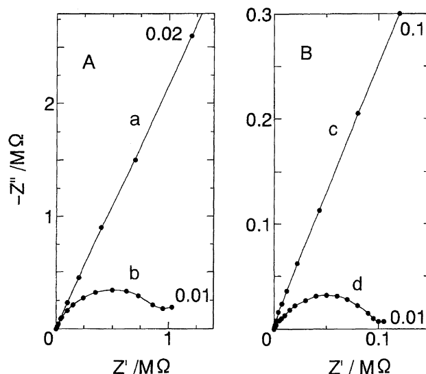
Fig. 4. Typical complex plane impedance diagrams of naked GC electrode (A) and poly-MPP-coated GC electrode (B) in the absence (a, c) and the presence (b, d) of quinhydrone in a 0.2 M Na 2 SO 4 –0.01 M H 2 SO 4 solution. Applied potential: 0.36 V. Numerical values in the figure exhibit frequencies in Hz.
